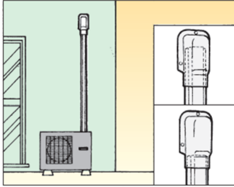
Cover the wall hole with duct cap
